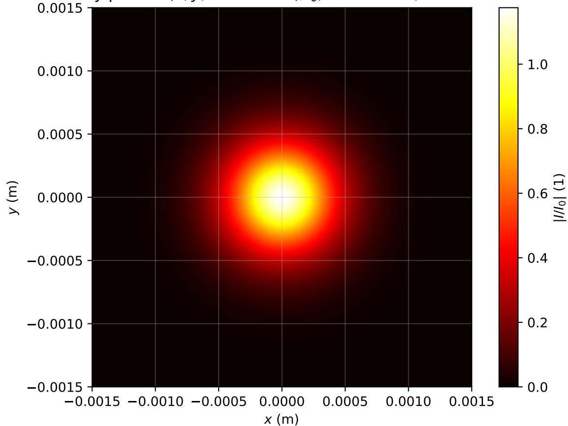
Intensity profile I(x, y, z = 0.557m)/I_0 , Pin=0.9Pcr, artificial time
